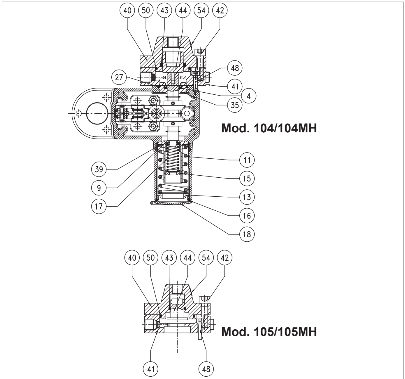
Fig. 9.30. Pressostato Mod. 104M/104MH - 105M/105MH
