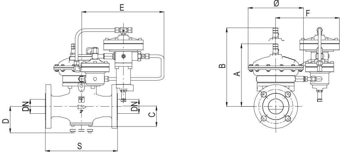
Figure 7 Dixi dimensions
