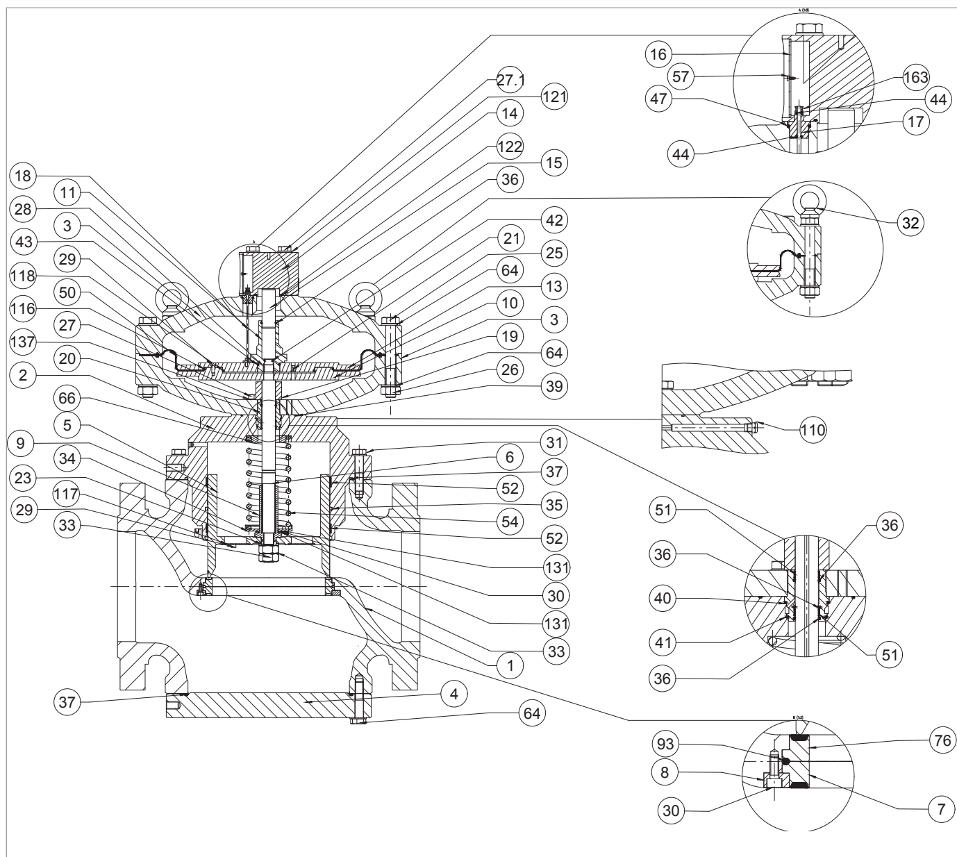
Regulator REFLEX 819 12"
