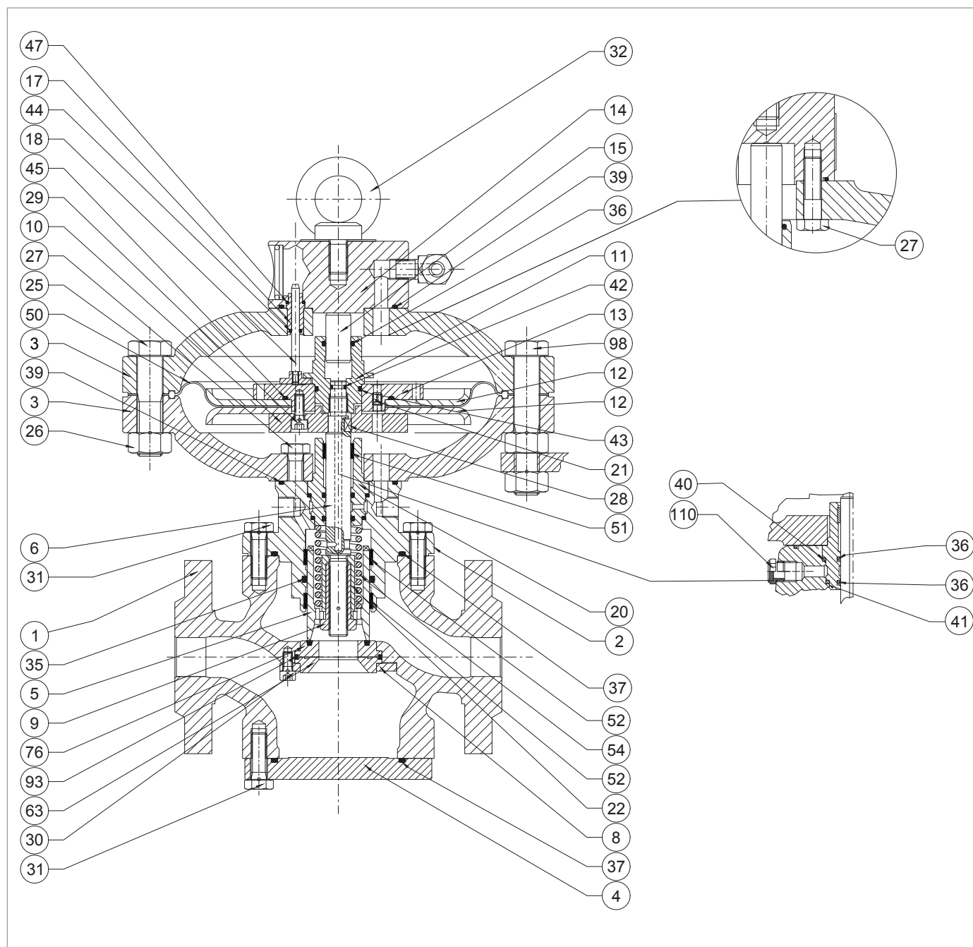
Regulator REFLEX 819 1" ÷ 2"
