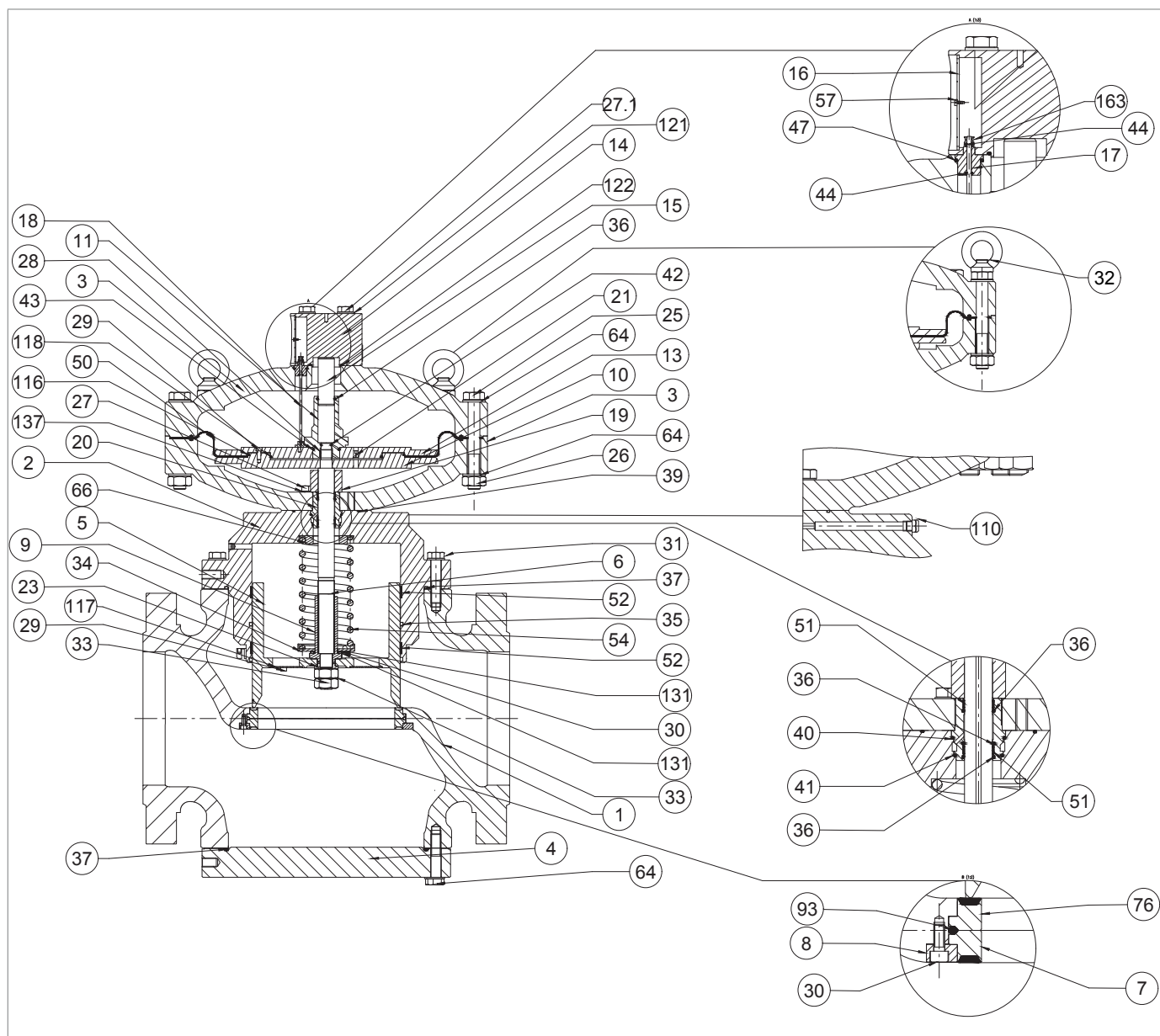
Rys. 9.59. Regulator REFLUX 819 12"
