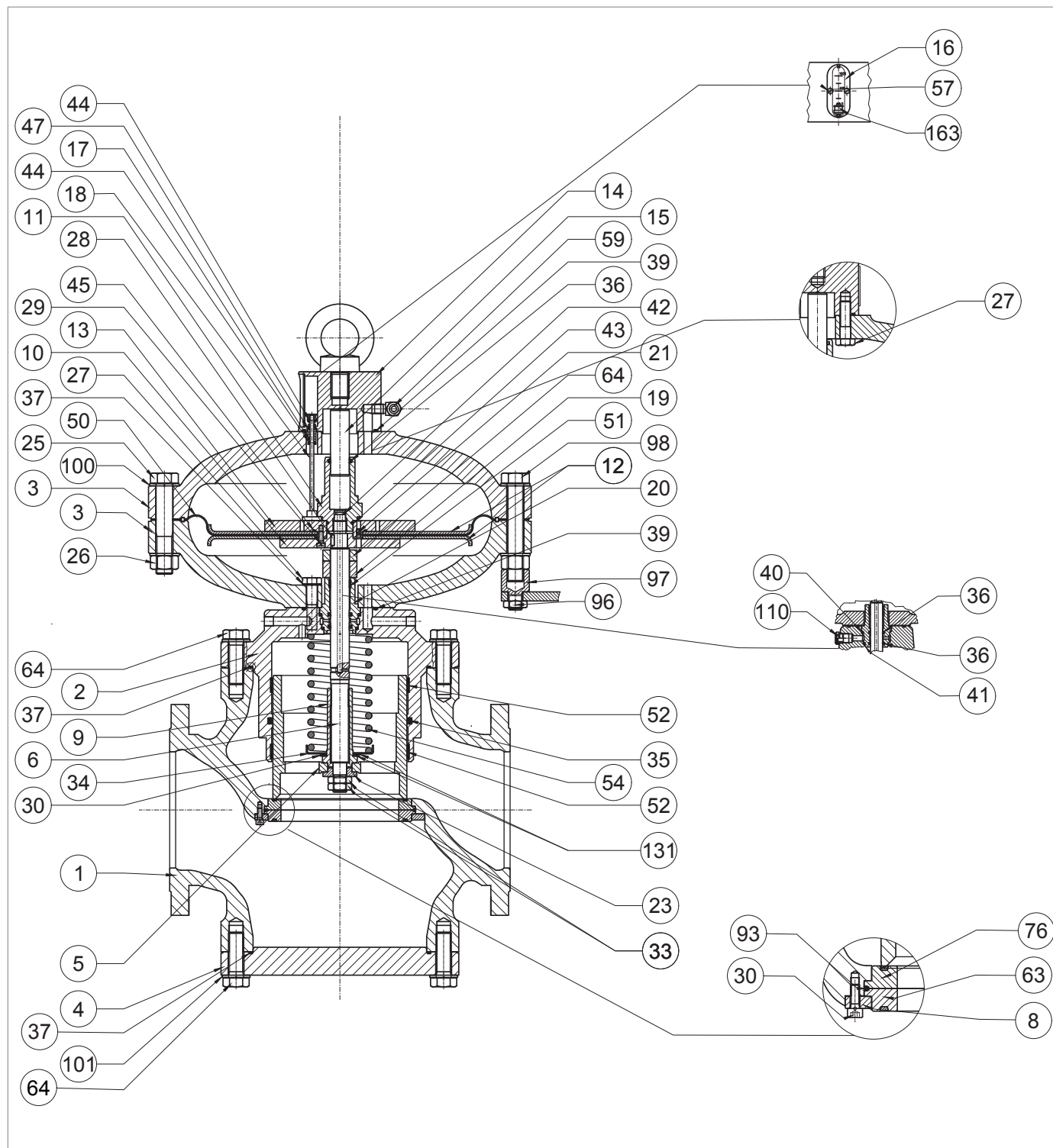
Regulator REFLEX 819 6" ÷ 8"
