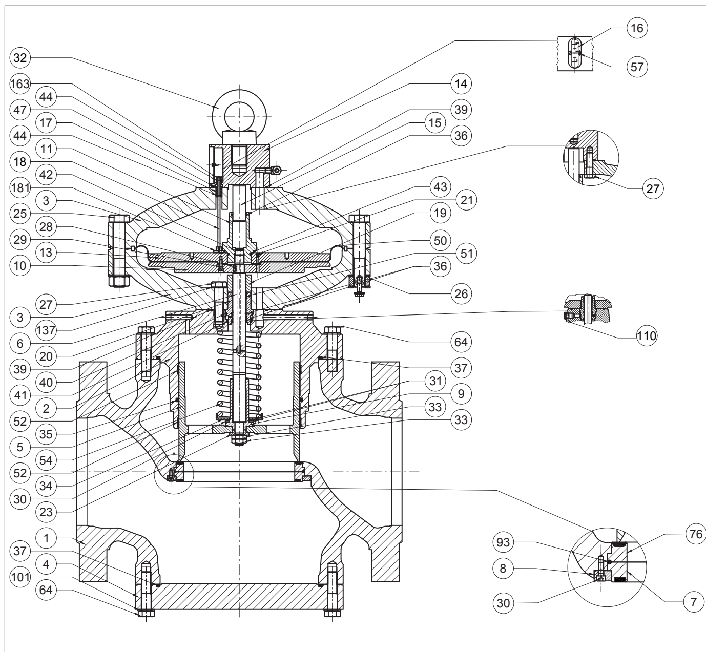
Rys. 9.58. Regulator REFLUX 819 10"
