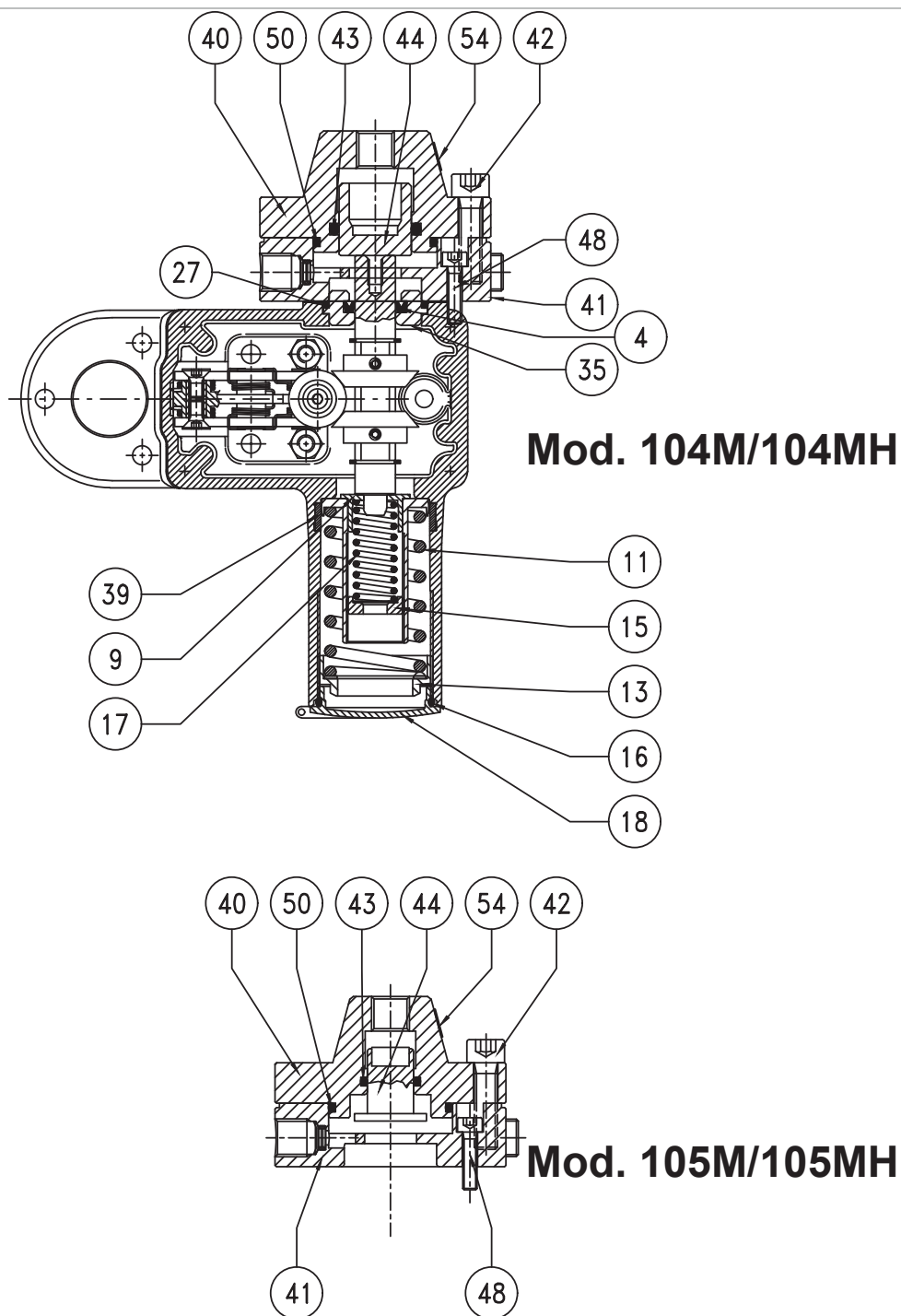
Rys. 9.76. Presostat Mod. 104M/104MH ÷ 105M/105MH
