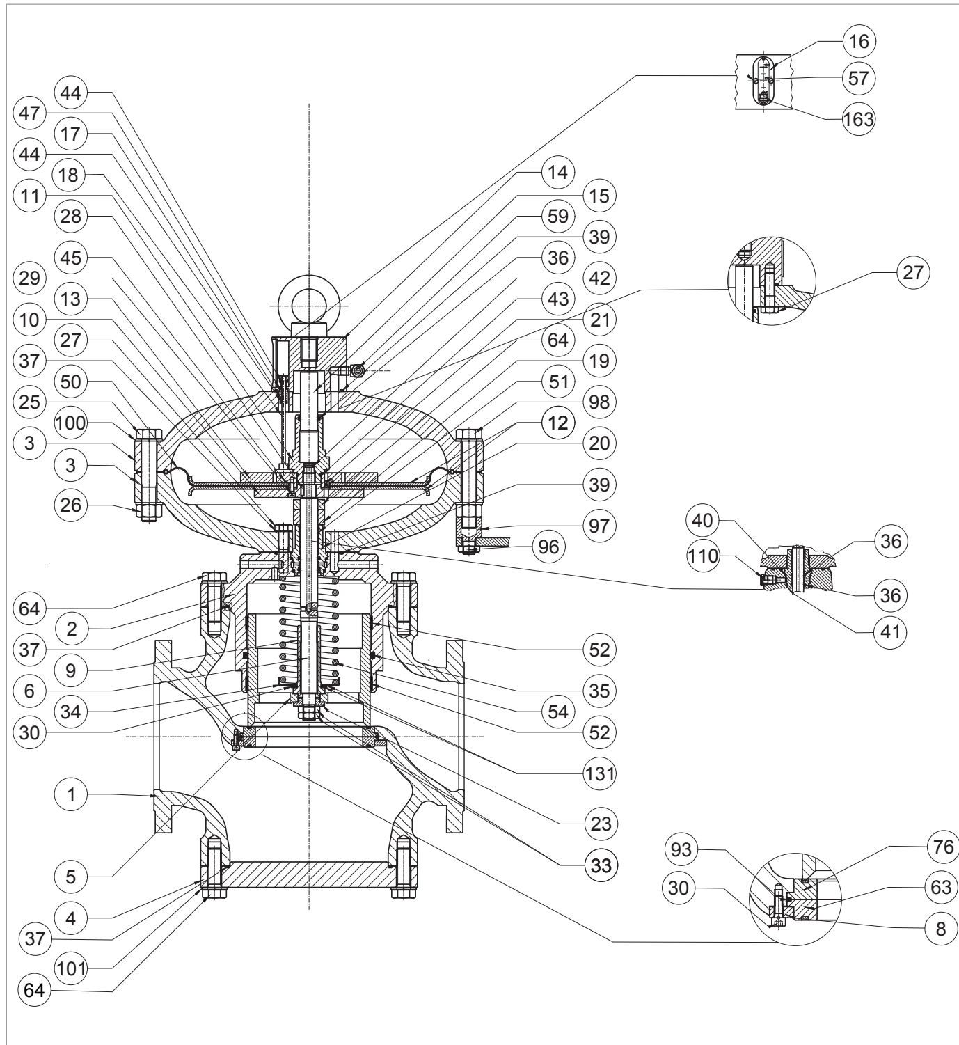
Regulator REFLEX 819 6" ÷ 8"
