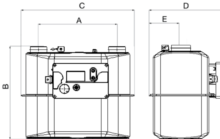
Figure 9 HM-iCON dimensions
